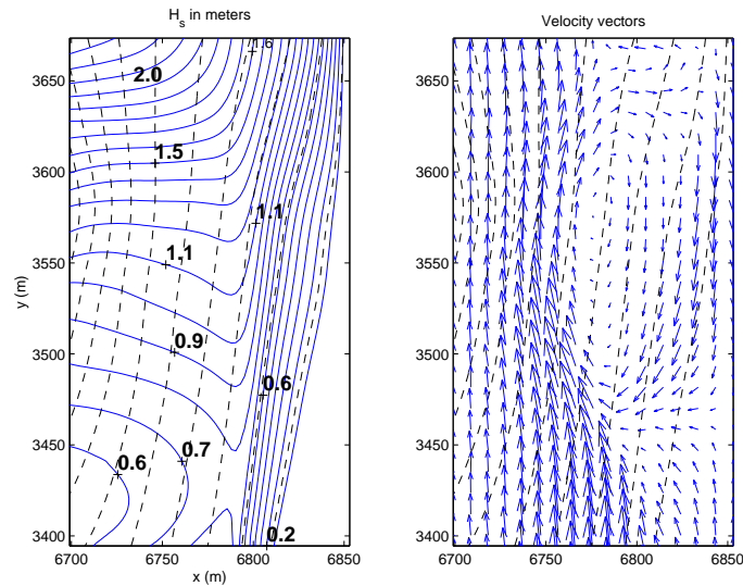
Figure 5: Waves and currents over nearshore grid, Scripps Canyon. Left: H_{1/3} . Right: Current vectors; the longest vector corresponds to 1 m/s .
