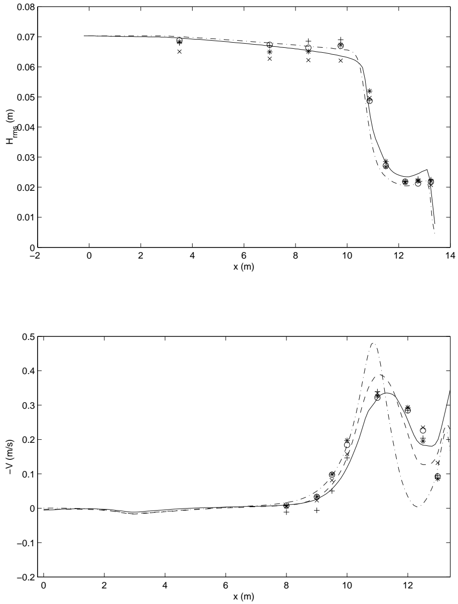
Figure 1: Comparison to experiment of Reniers and Battjes (1997). Top: H_{rms} ; solid line: Battjes and Janssen decay; dashed line: Thornton and Guza decay. Bottom: Longshore current; solid line: Battjes and Janssen decay with Stive and deVriend roller; dashed line: Thornton and Guza decay with Stive and deVriend roller; dashed-dot line: Thornton and Guza decay with static roller. Symbols indicate measurements.
