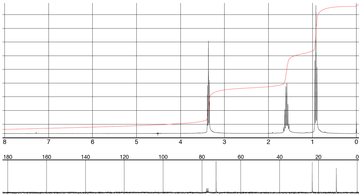
Compound 4: C 6 H 14 O
