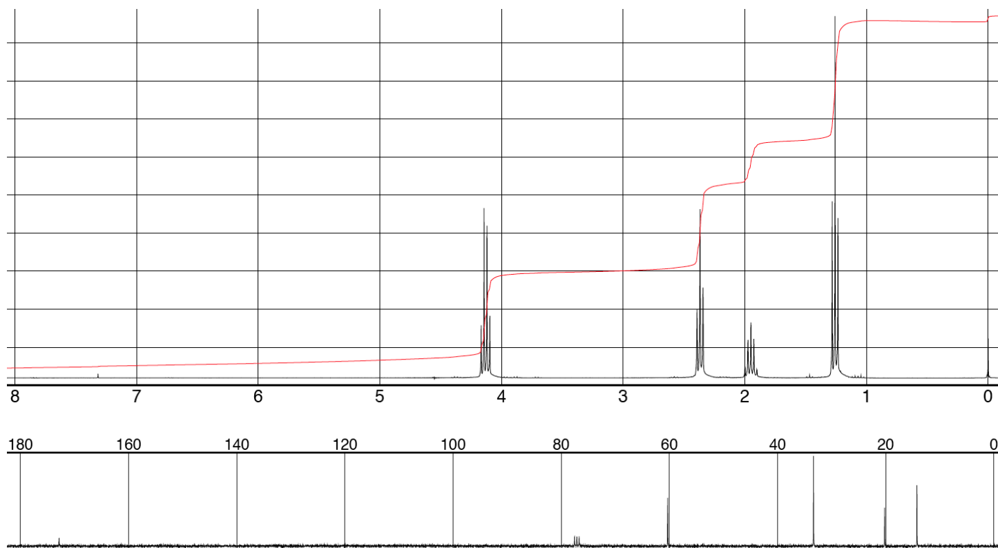
Compound 3: C 9 H 16 O 4
