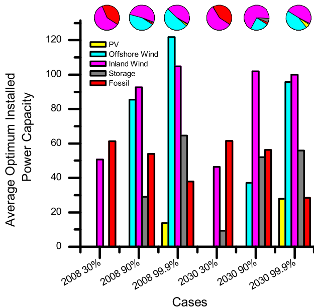
Fig. 5. Power capacity of generation and storage (bars) and source of energy used to meet load (pie charts) in all 18 RREEM runs. Each cluster of bars (e.g. the 4 bars labeled “2008 90%”) and pie chart above are an average of the three storage technologies.
