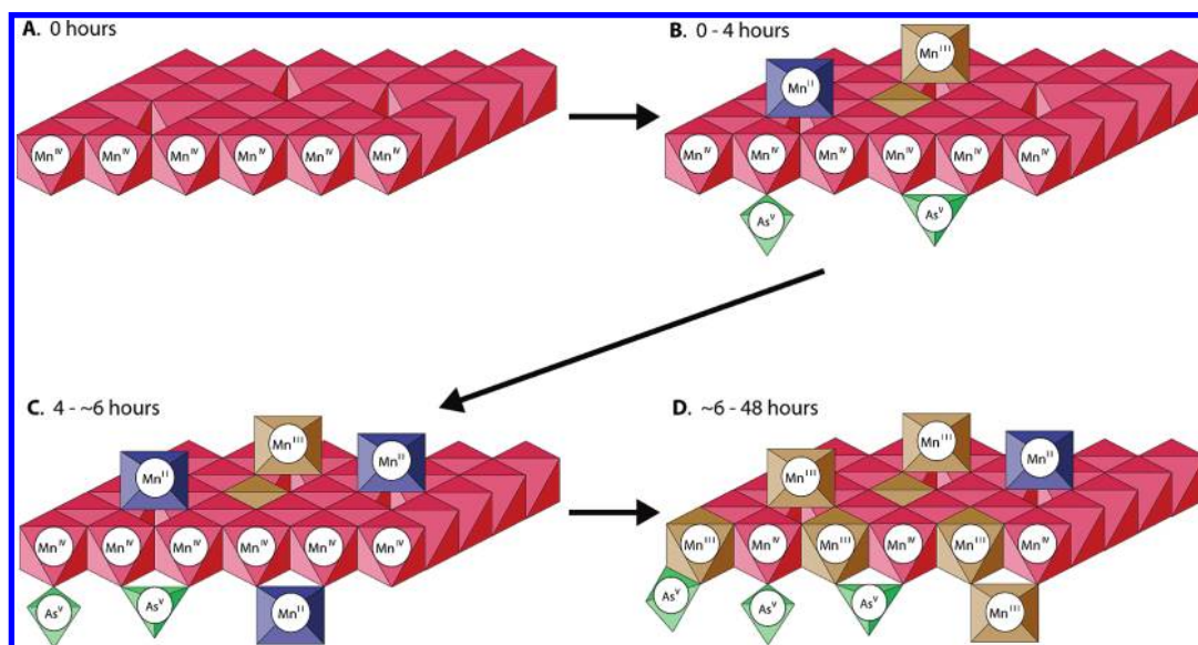
FIGURE 4. Proposed reaction mechanism for \text{As}^{\text{III}} oxidation by \delta\text{-MnO}_2 over 48 h in a stirred-flow reactor. Throughout the reaction, \text{As}^{\text{III}} is oxidized by \text{Mn}^{\text{IV}} at \delta\text{-MnO}_2 edge sites, producing \text{Mn}^{\text{II}} and \text{As}^{\text{V}} . (A) Unreacted \delta\text{-MnO}_2 octahedral layers consist of primarily \text{Mn}^{\text{IV}} and have reaction sites at layer edges (edge sites) and vacancy sites. (B) During the first 4 h of \text{As}^{\text{III}} oxidation, \text{Mn}^{\text{II}} sorbs at \delta\text{-MnO}_2 vacancy sites, and \text{As}^{\text{V}} sorbs at edge sites in bidentate–binuclear and monodentate–mononuclear complexes. Also, a portion of sorbed \text{Mn}^{\text{II}} reacts with \text{Mn}^{\text{IV}} at vacancy sites to form \text{Mn}^{\text{III}} . (C) Between 4 and \sim 6 h of reaction, vacancy sites become filled with \text{Mn}^{\text{III}} , \text{Mn}^{\text{II}} begins to sorb at \delta\text{-MnO}_2 edge sites, and \text{As}^{\text{V}} sorption continues in the same sorption complexes. (D) Beyond \sim 6 h of reaction, \text{Mn}^{\text{II}} at edge sites (and probably vacancy sites) reacts with \text{Mn}^{\text{III}} in \delta\text{-MnO}_2 octahedral layers to form \text{Mn}^{\text{III}} . The resulting \text{Mn}^{\text{III}} changes the bonding environment of \text{As}^{\text{V}} , which begins to sorb in bidentate–mononuclear complexes, and the As–Mn distance in \text{As}^{\text{V}} bidentate–binuclear complexes increases slightly.
