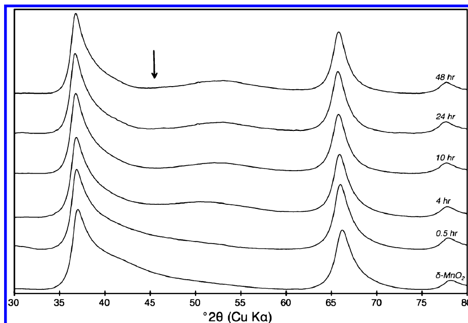
FIGURE 2. Synchrotron XRD patterns of unreacted \delta -MnO 2 and \delta -MnO 2 (1 mg/L) reacted with As III (100 \mu M) in a stirred-flow reactor for 0.5, 4, 10, 24, and 48 h. Arrow indicates the position of the 'dip' at 45° that increases with reaction time.
