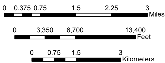
Tsunami sources modeled for Cape Hatteras, NGDC DEM
