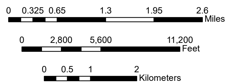
Tsunami sources modeled for Savannah, NGDC DEM
