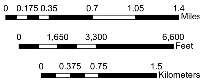
Tsunami sources modeled for Myrtle Beach, NGDC DEM
