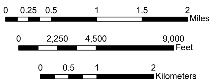
Tsunami sources modeled for Virginia Beach, NGDC DEM
