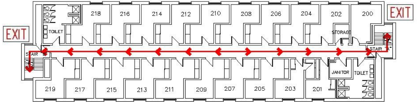
2nd - 3rd Floors Evacuation Map
