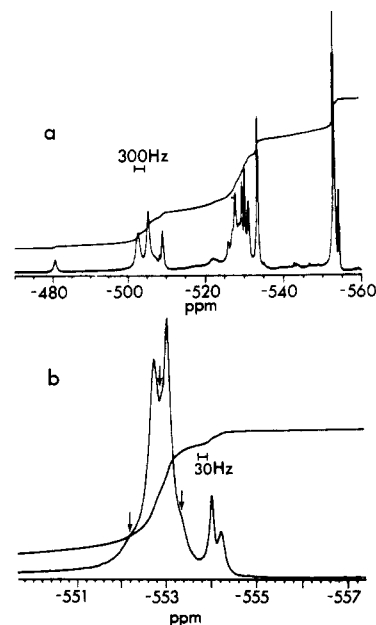
Figure 9. (a) 131.4-MHz ^{51}\text{V} NMR spectrum of \text{K}_6\text{V}_3\text{W}_9\text{O}_{40} (pH 4). (b) Expansion of the region between -550 and -557 ppm. Arrows indicate unresolved shoulders.
