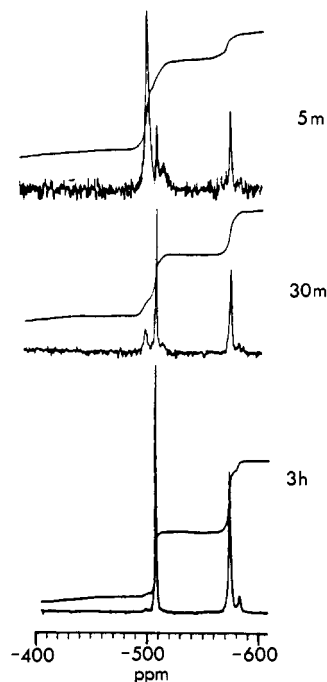
Figure 2. 23.67-MHz ^{51}\text{V} NMR spectra of \text{Na}_3\text{V}_3\text{W}_3\text{O}_{19} recorded at different times from the preparation of the solution (pH 7.5, 30^\circ\text{C} ).
