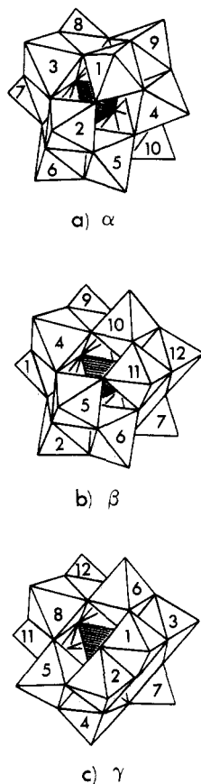
Figure 3. IUPAC numbering of metal atom positions in \alpha , \beta , and \gamma isomers of the Keggin anion.
