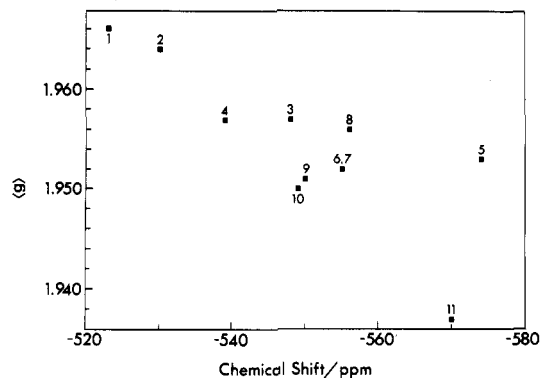
Figure 12. \langle g \rangle for metalovanadates(IV) vs. \delta(^{51}\text{V}) for the corresponding metalovanadates(V). Anions: (1) \text{VW}_5\text{O}_{19}^{3-} ; (2) \alpha\text{-PVMo}_{11}\text{O}_{40}^{4-} ; (3) \alpha\text{-SiVW}_{11}\text{O}_{40}^{5-} ; (4) \text{H}_2\text{VW}_{11}\text{O}_{40}^{7-} ; (5) \alpha\text{-BVW}_{11}\text{O}_{40}^{6-} ; (6) \alpha\text{-PVW}_{11}\text{O}_{40}^{4-} ; (7) \alpha_2\text{-P}_2\text{VW}_{17}\text{O}_{62}^{7-} ; (8) \beta_1\text{-SiVW}_{11}\text{O}_{40}^{5-} ; (9) \beta_2\text{-SiVW}_{11}\text{O}_{40}^{5-} ; (10) \beta_3\text{-SiVW}_{11}\text{O}_{40}^{5-} ; (11) \alpha_1\text{-P}_2\text{VW}_{17}\text{O}_{62}^{7-} .
