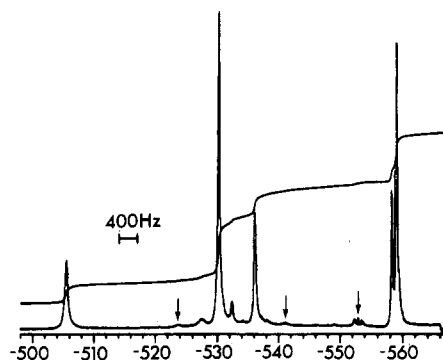
Figure 7. 131.4-MHz ^{51}\text{V} NMR spectrum of \text{K}_5\text{VV}_2\text{W}_{10}\text{O}_{40} (pH 2.0). The arrows indicate the impurity of \text{VV}_3\text{W}_5\text{O}_{40}^{6-} .
