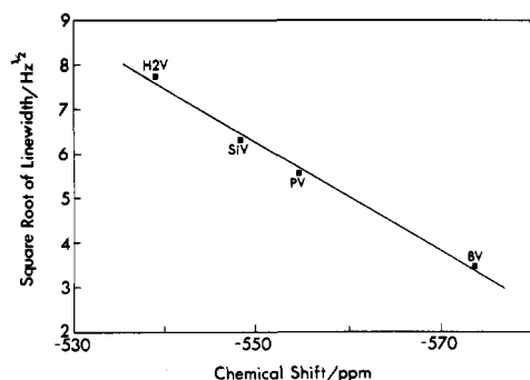
Figure 10. Plot of the square root of the line width vs. ^{51}\text{V} chemical shift for \alpha\text{-RVW}_{11}\text{O}_{40}^{m-} anions.
