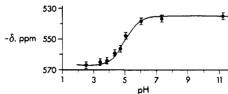
Figure 4. Plot of \delta(^{51}\text{V}) vs. pH for \alpha -1,2,3- \text{SiV}_3\text{W}_9\text{O}_{40}^{7-} . The line was calculated for \text{pK}_a = 4.97 .
