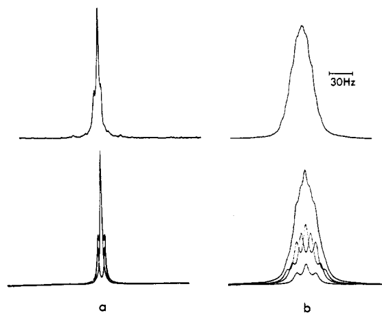
Figure 1. (a) 23.67-MHz 51 V NMR spectrum of (Bu 4 N) 3 VW 5 O 19 in CD 3 CN at 80^\circ\text{C} (upper) and the simulated spectrum (lower). (b) 78.9-MHz 51 V NMR spectrum of (Bu 4 N) 3 VW 5 O 19 , enriched with 82.5% 183 W, in CD 3 CN at 80^\circ\text{C} (upper) and the simulated spectrum (lower).
