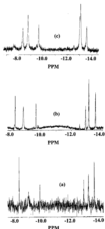
Figure 5. ^{31}\text{P} NMR spectra taken at 296 K for the mixtures formed by 2-electron reduction of \text{K}_{16}[\text{Th}(\alpha_2\text{-P}_2\text{W}_{17}\text{O}_{61})_2] solutions of various concentrations in 1 M lithium acetate buffer (pH = 4.7), containing 20% \text{D}_2\text{O} for lock: (a) 0.5 mM; (b) 2.0 mM; (c) 5.0 mM.
