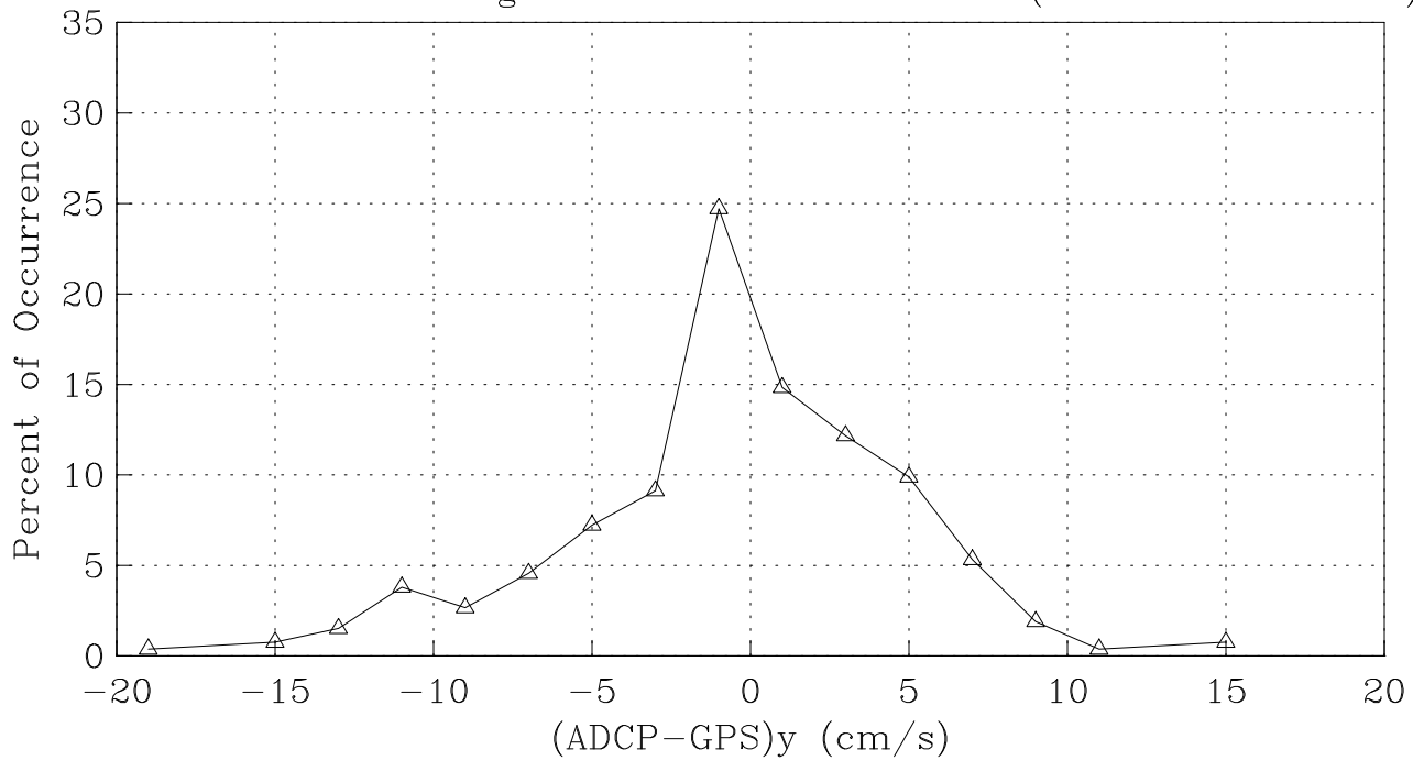
SBI-2004 Fall Mooring Cruise ADCP Calibration (09-12-2004 amue)
