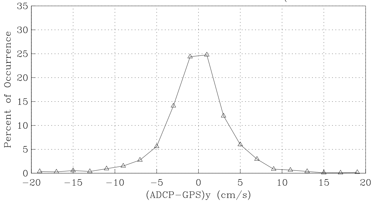
SBI-2004 Summer Process Cruise ADCP Calibration (09-12-2004 amue)
