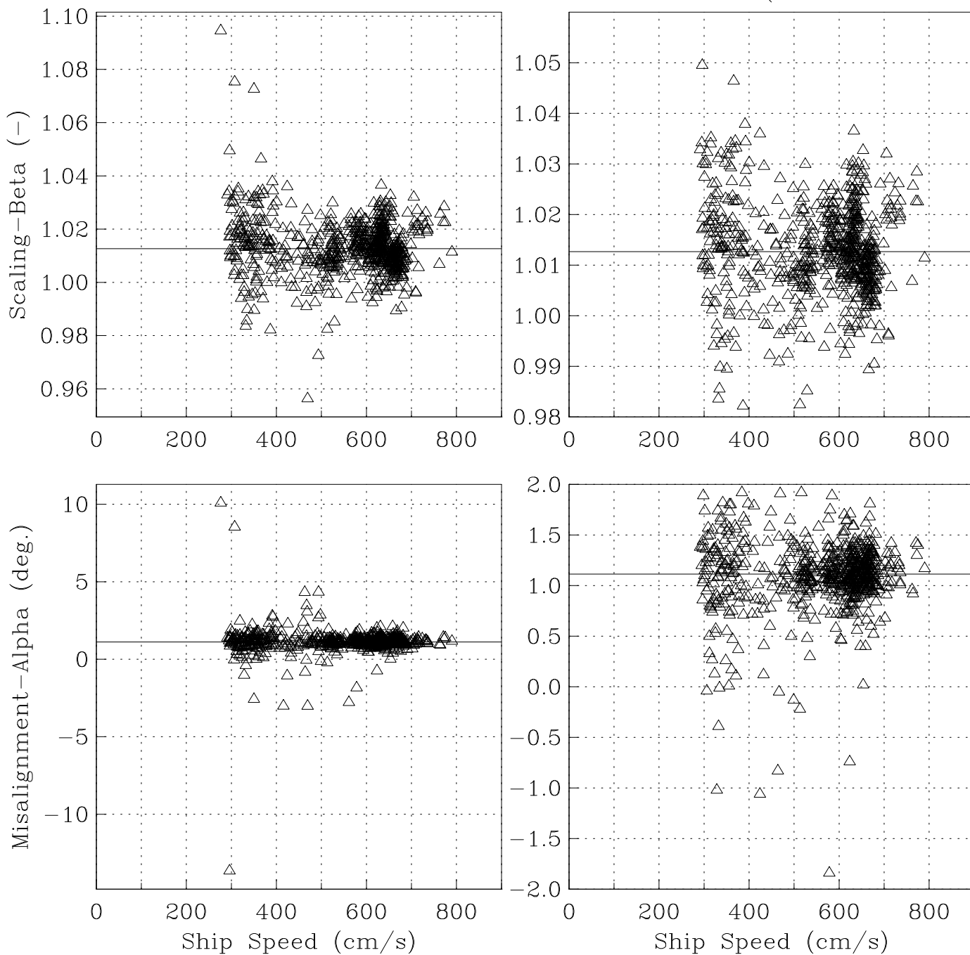
SBI-2004 Summer Process Cruise ADCP Calibration (09-12-2004 amue)
