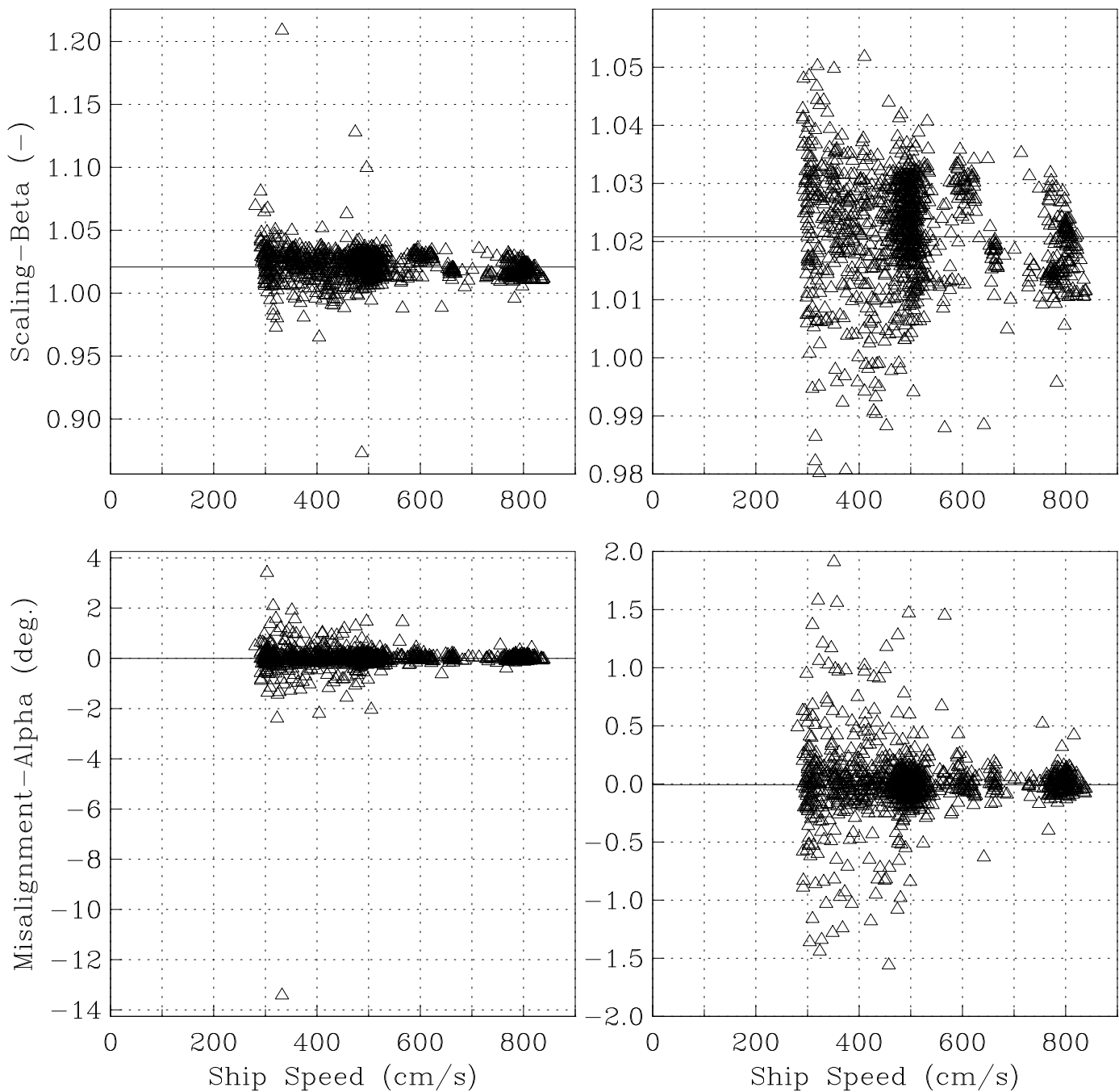
SBI-2003 Fall Mooring Cruise ADCP Calibration (09-12-2004 amue)
