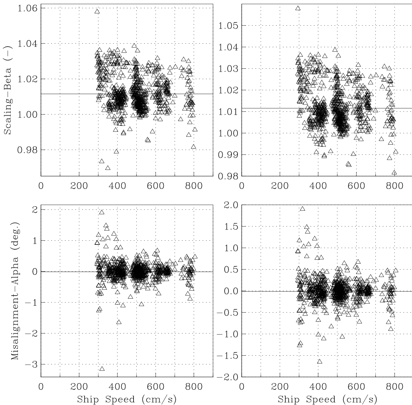
SBI-2002 Summer Process Cruise ADCP Calibration (10-18-2004 amue)
